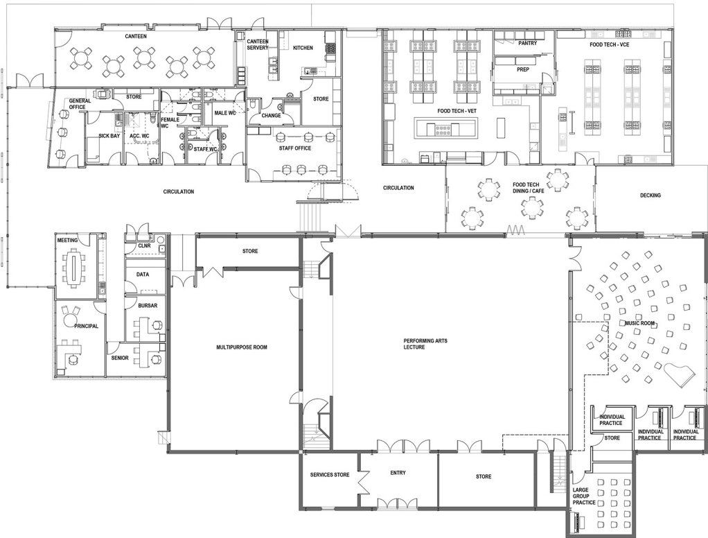
1 GENERAL ARRANGEMENT PLAN - SENIOR SCHOOL - OVERALL 1:500
