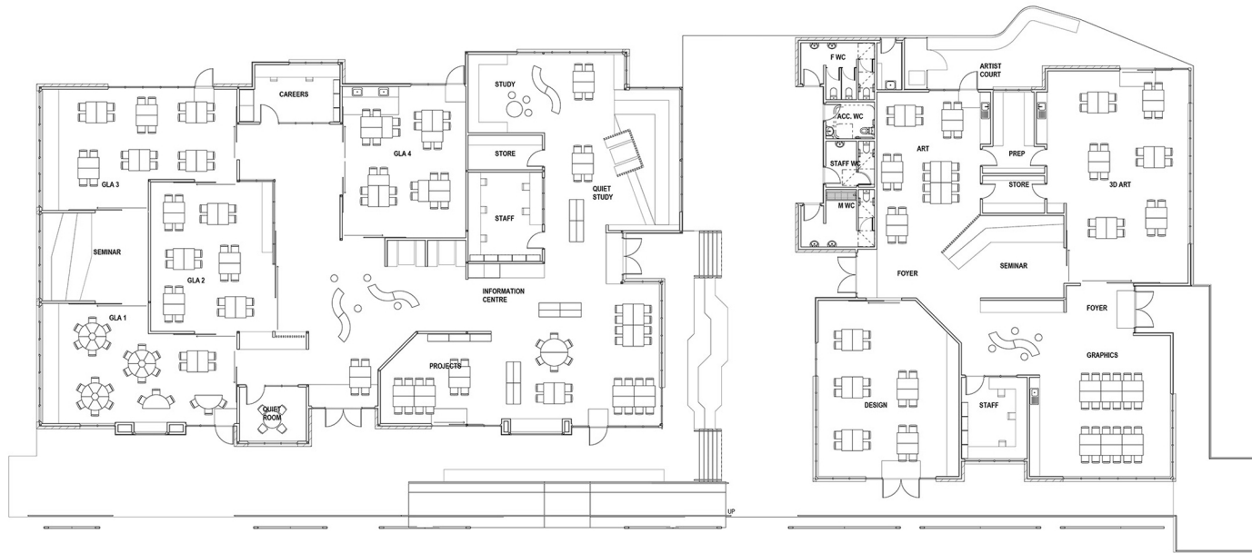
1 GENERAL ARRANGEMENT PLAN - SENIOR SCHOOL - OVERALL 1:500
